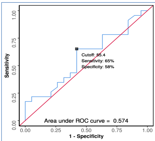
Figure 2: ROC curve analysis showing diagnostic performance of CA125 (U/ml) in predicting metastatic GBC vs locally advanced (n=42).
