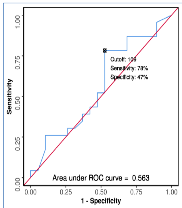
Figure 1: ROC curve analysis showing diagnostic performance of CA-19-9 (U/ml) in predicting metastatic GBC vs locally advanced (n=42).
