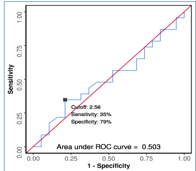
Figure 3: ROC curve analysis showing diagnostic performance of CEA ( \mu\text{g/l} ) in predicting metastatic GBC vs locally advanced (n=42).
